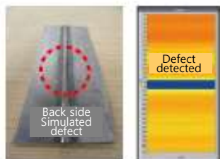
Butt welded of Steel plate (Left: Specimen, Right: Image by NAUT21)
