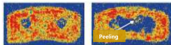
Brake Pad for Automobile - Image by NAUT21 (Left: Image of good brake pad, Right: Image of defective one)
