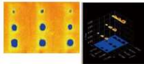
NAUT21-I Image (Left: Planar image by air coupled method) (Right: 3D image by immersion method)
