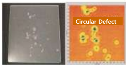
Contact Surface of Acrylic Resin (Left: Specimen, Right: Image by NAUT21)
